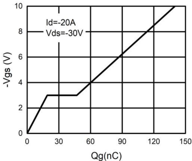
Fig.5 - Gate charge
