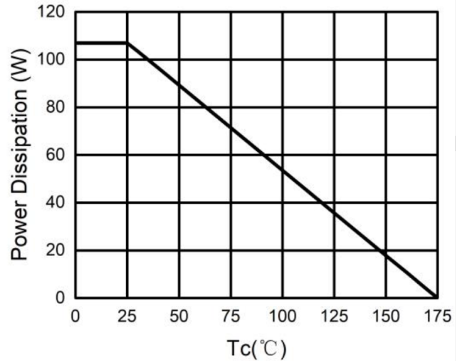
Fig.8 - Power Derating
