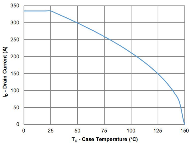
Fig.11 - Current Derating
