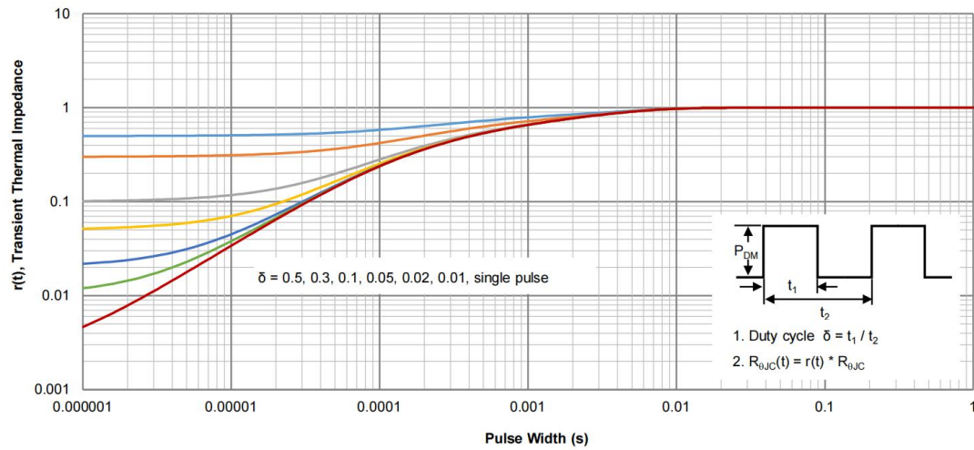
Fig.13 - Normalized Maximum Transient Thermal Impedance
