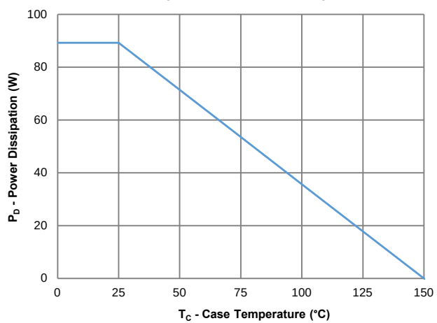
Fig.10 - Power Derating
