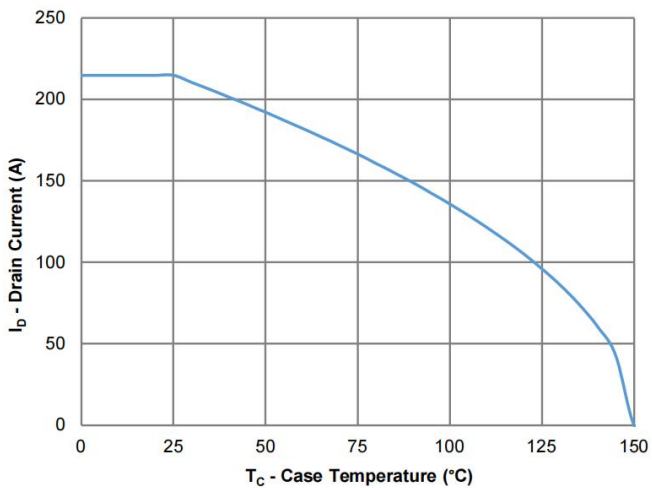
Fig.11 - Current Derating
