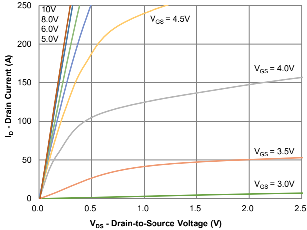
Fig.1 -Output Characteristics
