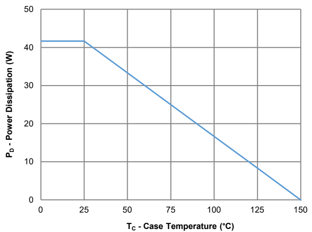
Fig.10 -Power Derating
