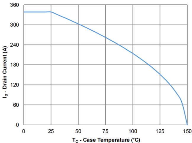
Fig.11 - Current Derating
