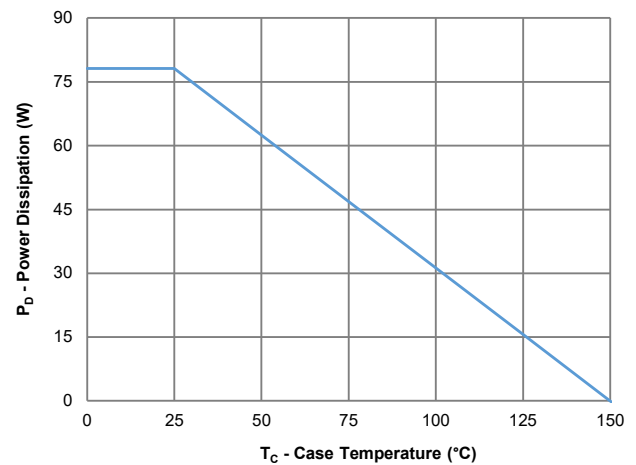
Fig10 - Power Derating
