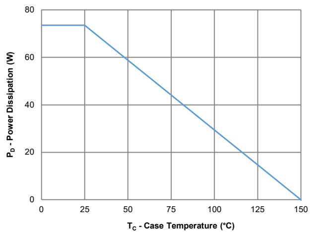
Fig10 - Power Derating
