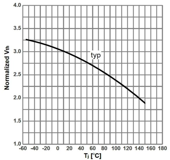
Fig.6 - Normalized Threshold Voltage
