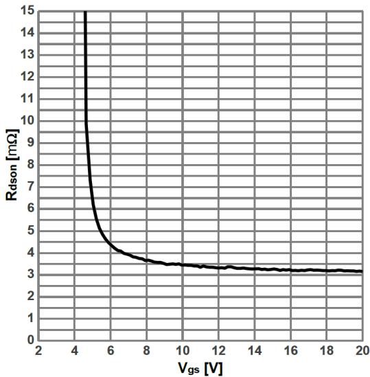
Fig.5 - Drain-Source On-Resistance
