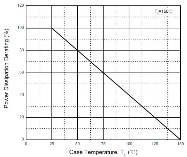
Fig.12 - Power Derating
