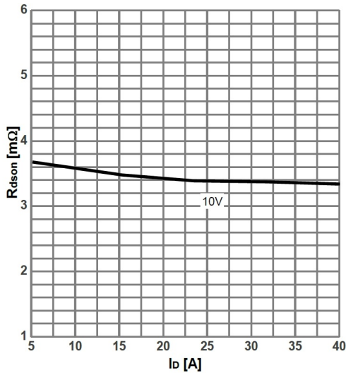
Fig.5 - Drain-Source On-Resistance
