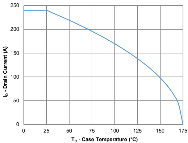
Fig11 - Current Derating
