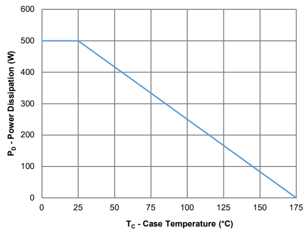
Fig10 - Power Derating
