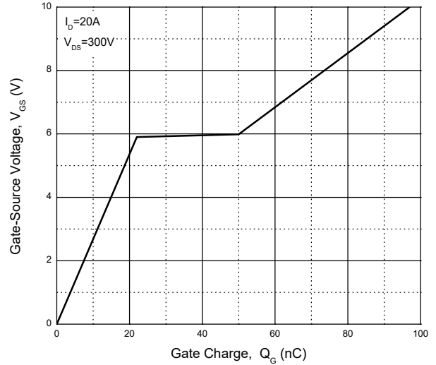
Fig. 8 - Gate Charge
