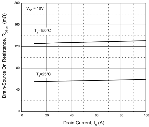
Fig. 3 - Drain-Source On-Resistance
