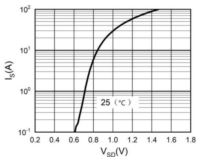
Fig.6 - Forward Characteristic
