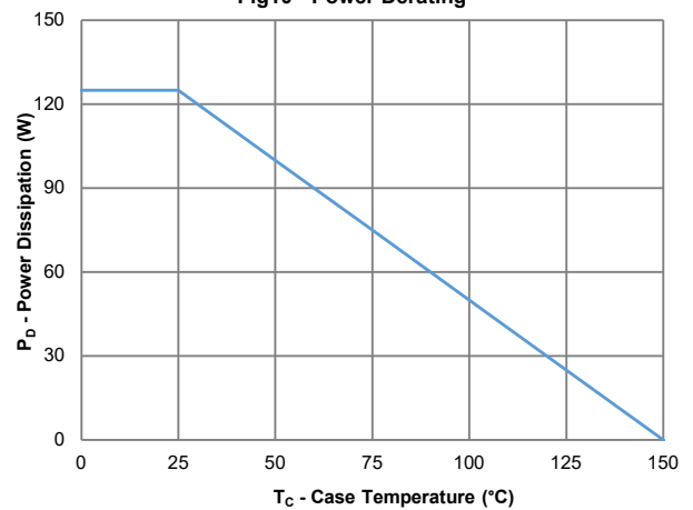
Fig10 - Power Derating
