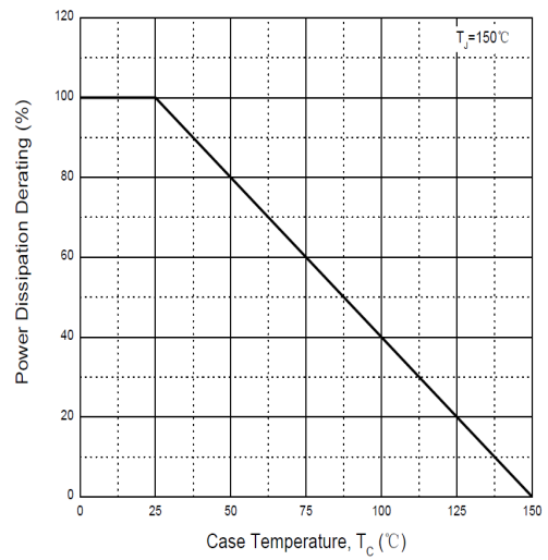
Fig.10 - Power Derating
