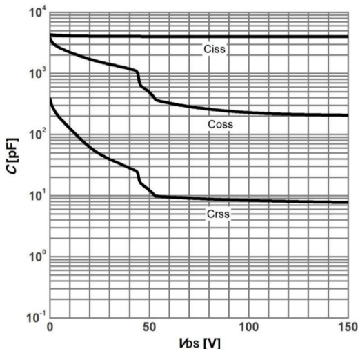
Fig.5 - Capacitance
