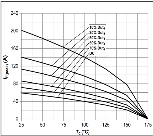
Fig.3 -Current Derating
